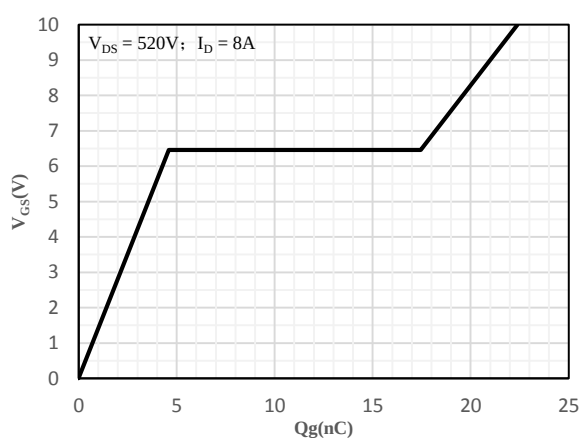
Fig 10 Gate-Charge Characteristics
